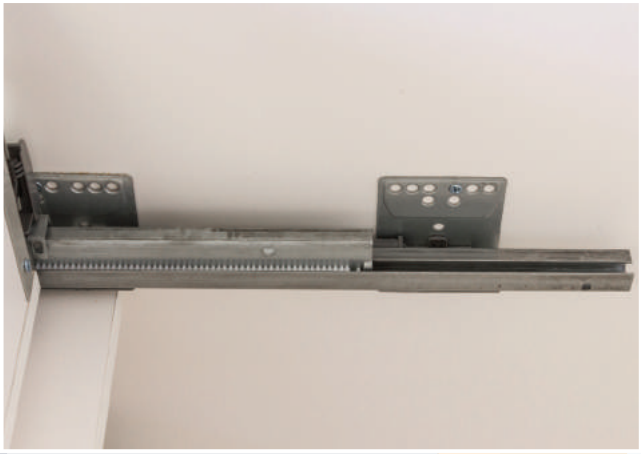
FULL EXTENSION - SELF CLOSING UNDER MOUNT RAILS
